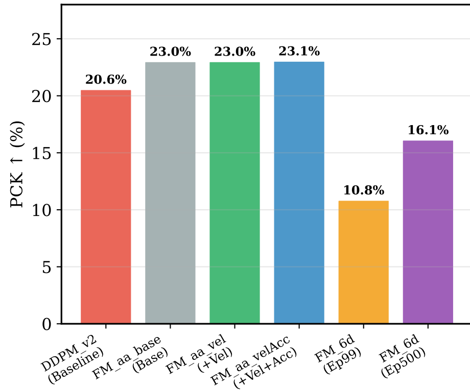
Joint Position Accuracy (PCK)
