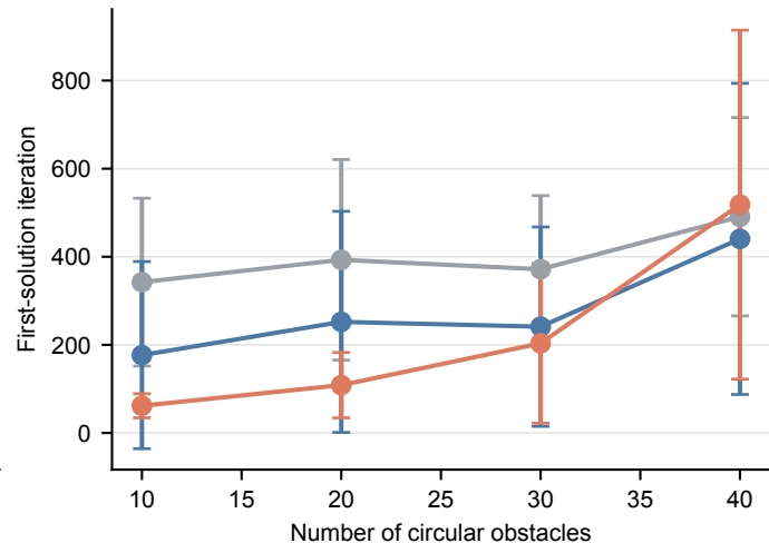
Density sensitivity of orchard path planners
