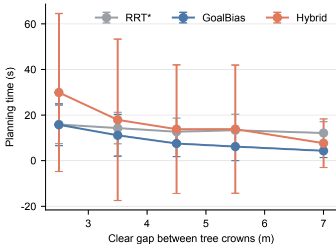
Clear-gap sensitivity of orchard path planners
