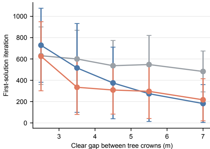
Clear-gap sensitivity of orchard path planners
