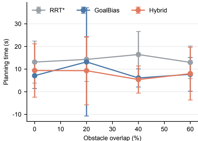
Overlap sensitivity of orchard path planners
