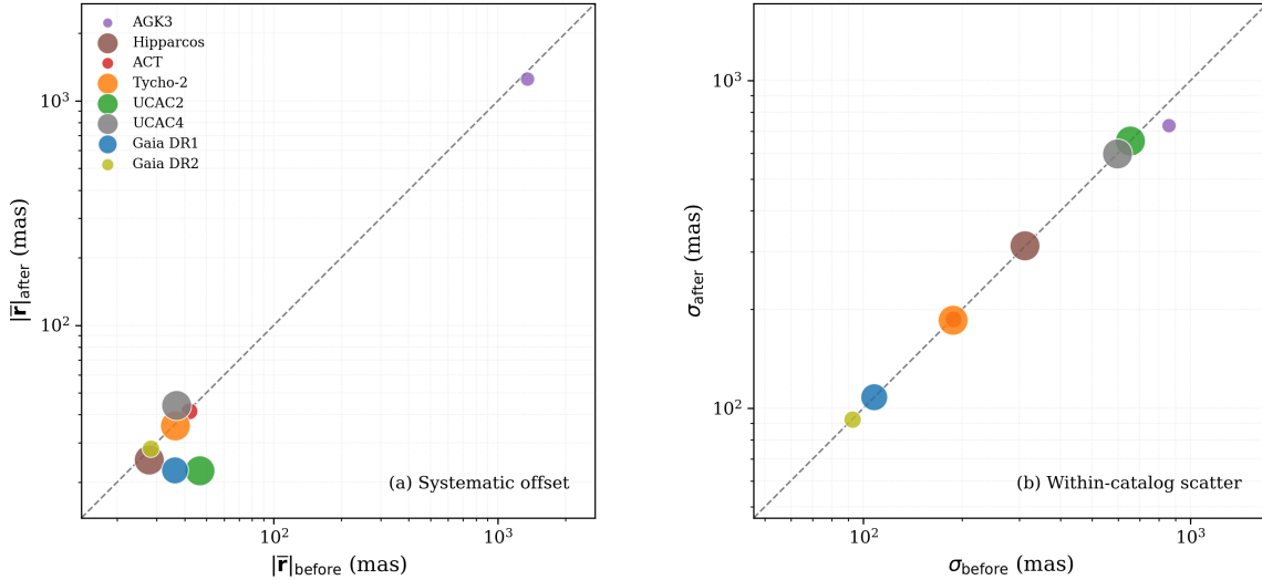
Figure 8. Catalog-level comparison of residual statistics before and after debiasing. (a) Systematic offset |\bar{r}| : points below the diagonal indicate reduced offsets. (b) Within-catalog scatter \sigma : clustering along the diagonal confirms that the random component is preserved. Point sizes scale with the number of observations; colors indicate the reference catalog.
