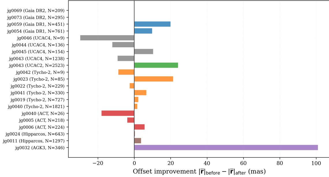
Figure 7. File-level improvement in systematic offset \Delta|\bar{r}| for each (file, catalog) group, ordered by catalog. Positive values indicate that the debiasing correction reduces the systematic offset with respect to the ephemeris.
