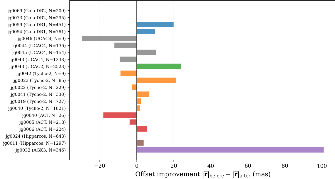
Figure 7. File-level improvement in systematic offset \Delta|\mathbf{F}| for each (file, catalog) group, ordered by catalog. Positive values indicate that the debiasing correction reduces the systematic offset with respect to the ephemeris.
