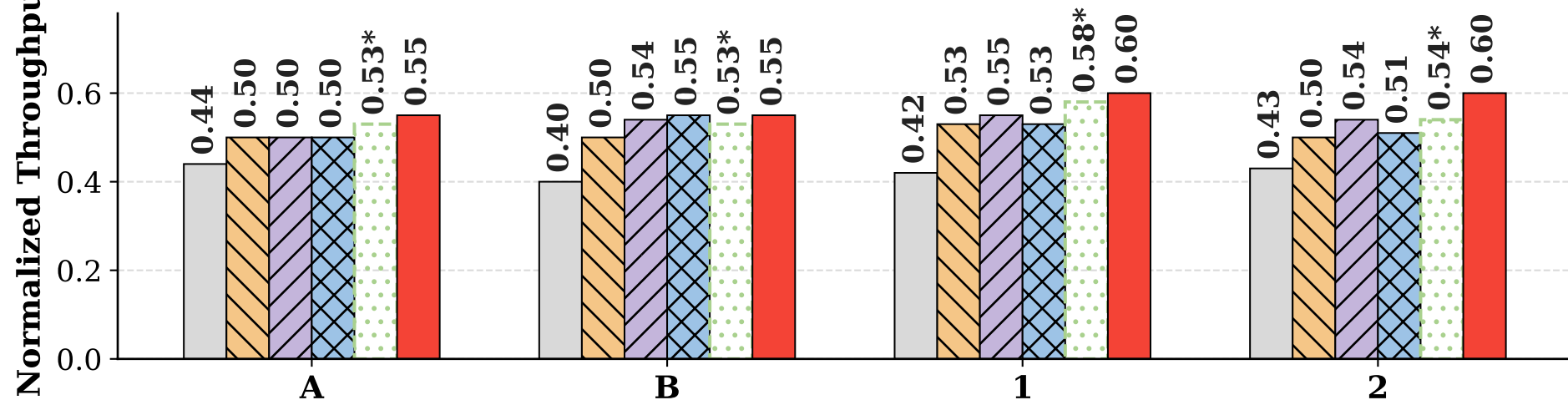
(a) DNN Training Job Performance (Higher is better)
