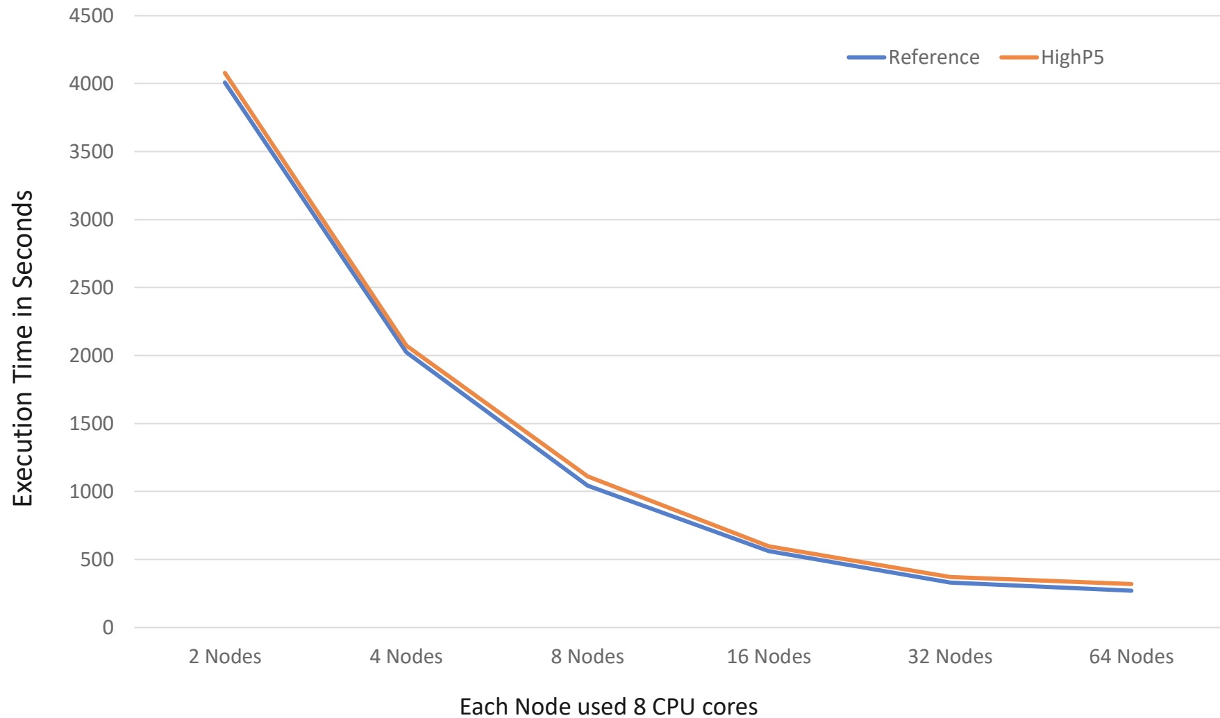
Conjugate Gradient with 51200^2 Square Matrix for 51200 Iterations
