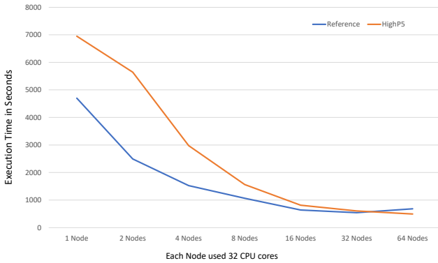
FIGURE 12 | Execution time comparison for block LU factorization of a 30720^2 Square Matrix for different number of nodes.
