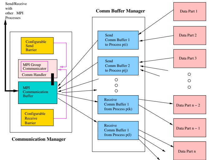
FIGURE 10 | The general architecture of a HighP5 communicator responsible for communicating array parts.
