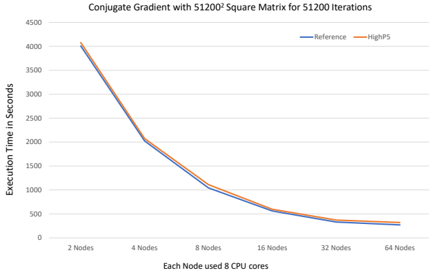
FIGURE 14 | Execution time comparison for conjugate gradient computation for a 95% sparse 51200^2 square matrix for 51200 iterations.
