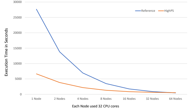
FIGURE 13 | Execution time comparison for finite difference calculation on a 204800 by 2048 rectangular plate using hundred thousand Jacobi iterations.
