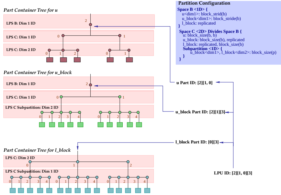
FIGURE 9 | An illustration of the process of retrieving data parts from Data Parts Registry using an LPU ID during block-LU factorization.
