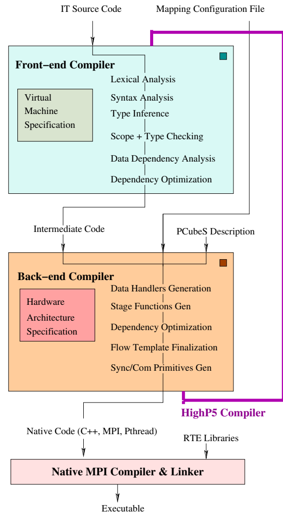
FIGURE 7 | Front-end/Back-end breakdown of the compiler.
