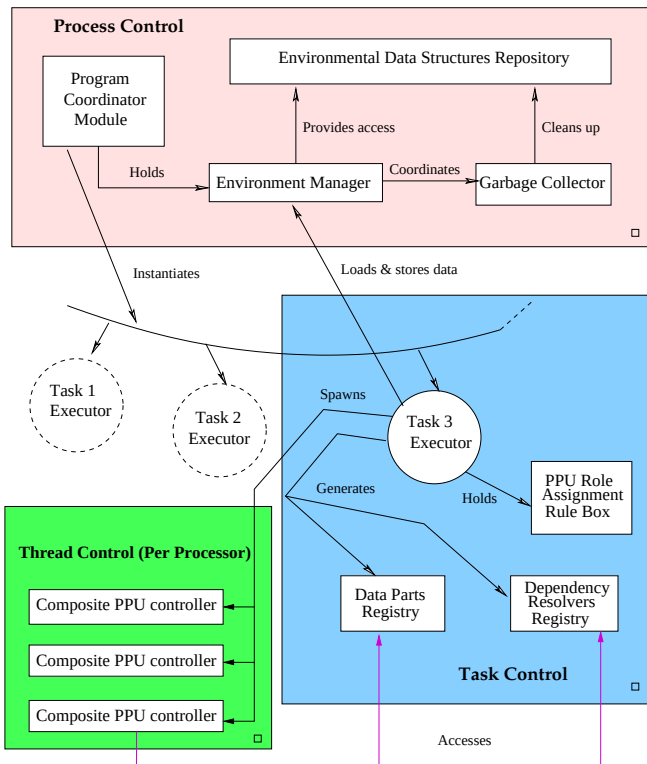
FIGURE 5 | The runtime process model of HighP5 executables.
