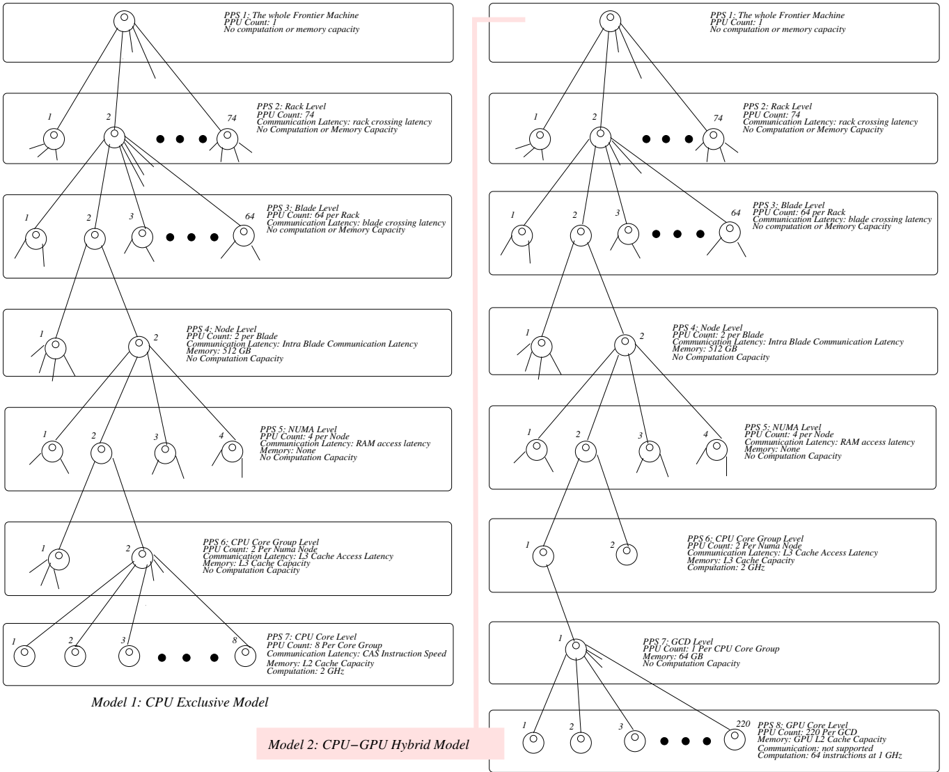
FIGURE 4 | An illustration of two PCubeS machine models of the Frontier Supercomputer. The depictions expand only one parallel processing unit at each level. Furthermore, details of the communication capacities (exact latencies and transaction bandwidth) have not been shown.
