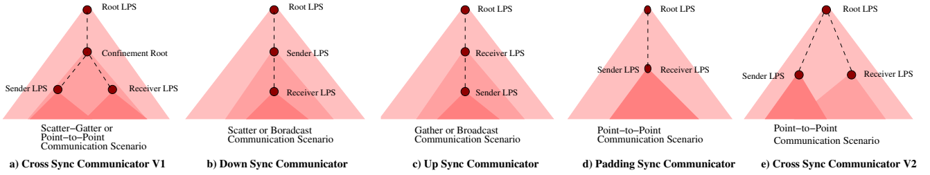
FIGURE 11 | An illustration of how relative positions of the LPSes in the LPS hierarchy involved in a data dependency determine the nature of MPI communication primitives.
