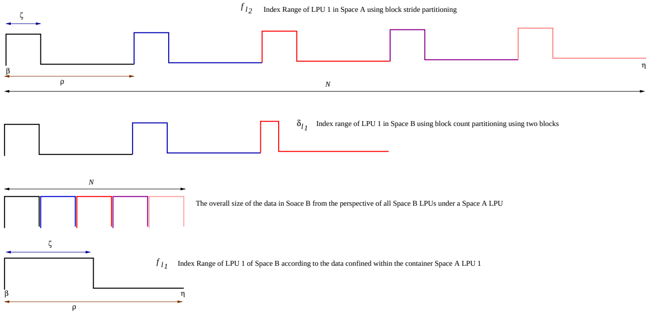
FIGURE 8 | An illustration of nested data partition using a two layer hierarchy where Space A is the upper and Space B is the lower LPS.
