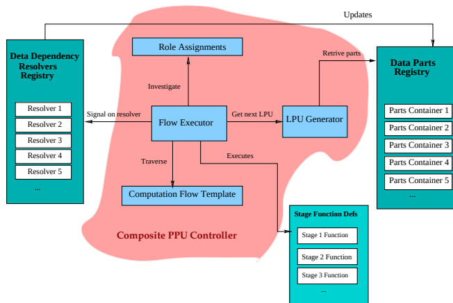
FIGURE 6 | The architecture of a composite PPU controller thread.
