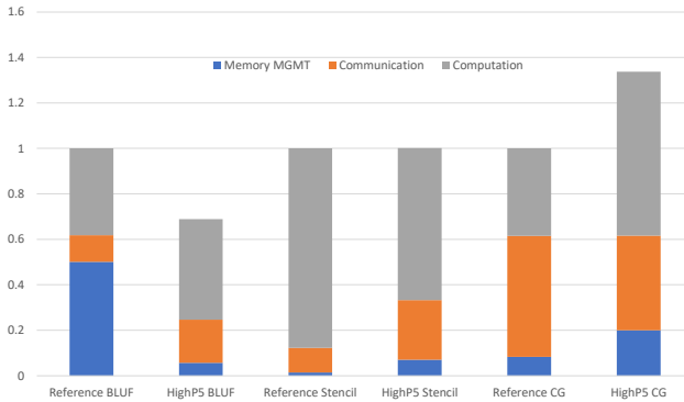
FIGURE 15 | Detail breakdown of the normalized execution times for three building block programs with large input sizes and 100 nodes scenario.
