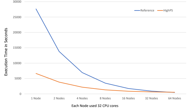
FIGURE 12 | Execution time comparison for finite difference calculation on a 204800 \times 2048 rectangular plate using hundred thousand Jacobi iterations.
