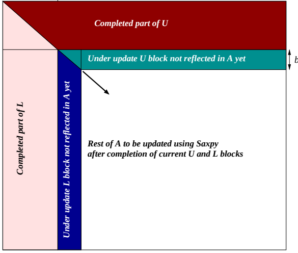
FIGURE 3 | An illustration of the progression of Block LU decomposition strategy.
