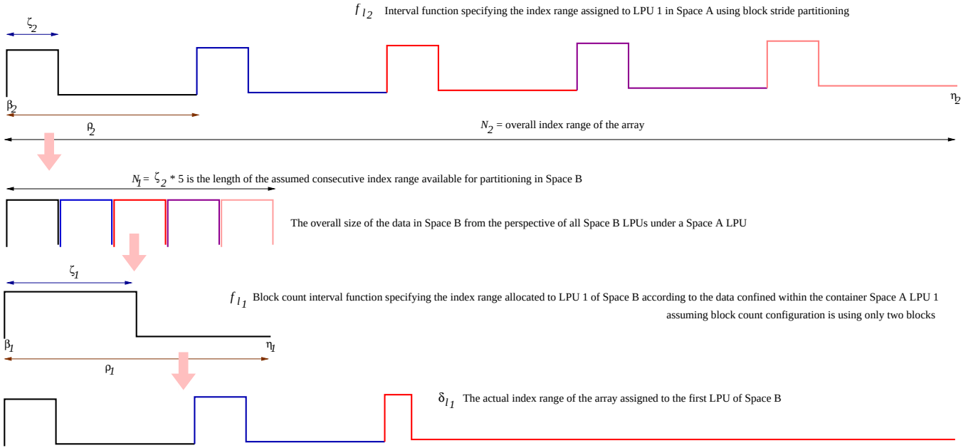
FIGURE 7 | An illustration of nested data partitioning using a two layer hierarchy where Space A is the upper and Space B is the lower LPS. The lower layer sees a compacted index space created by the upper layer's blocks.
