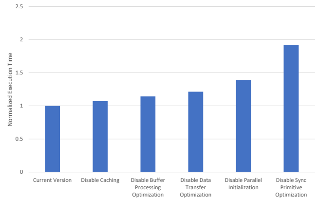
FIGURE 15 | Comparison of normalized execution times of different HighP5 executables for block LU factorization on 64 nodes.
