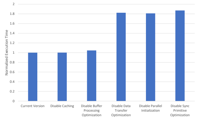
FIGURE 16 | Normalized execution times of different HighP5 iterative stencil executable versions for the 64 node scenario.
