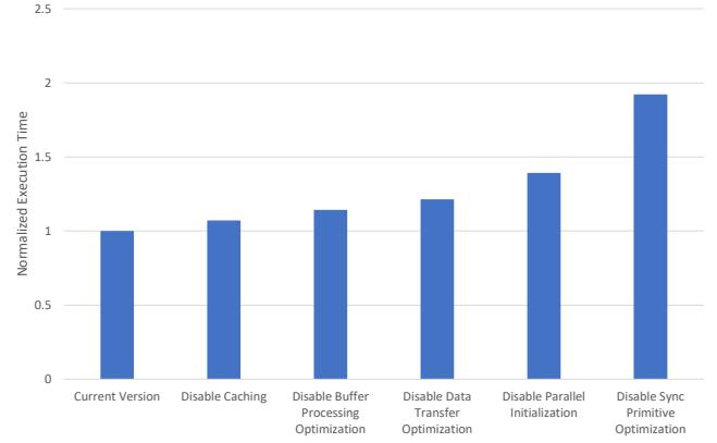
FIGURE 15 | Normalized execution times of different HighP5 block-LUF executable versions for the 64 node scenario.
