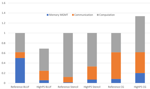
FIGURE 14 | Detail breakdown of the normalized execution times for three building block programs with large input sizes and 100 nodes scenario.
