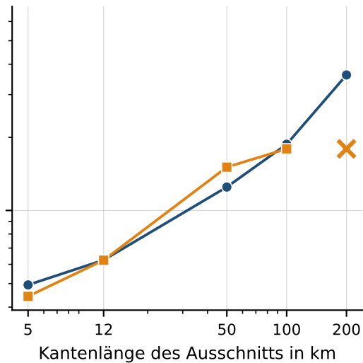
Terrascope
