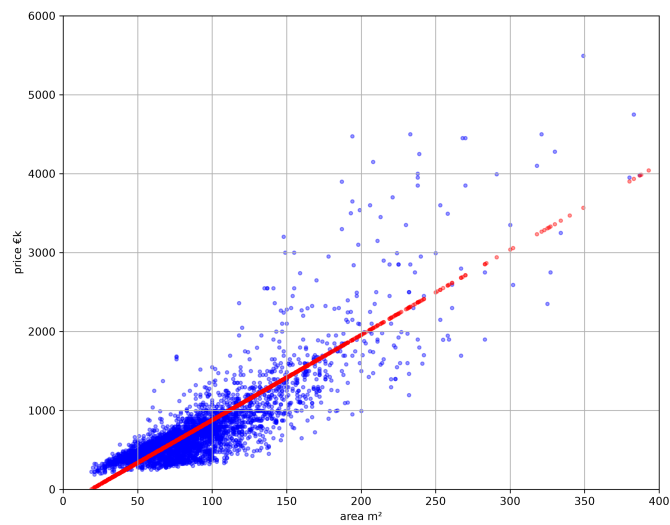
Figure 6: Model Results Without Outliers
