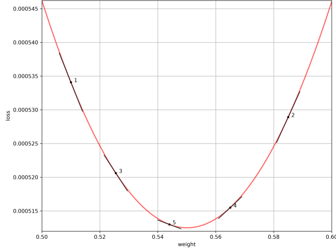
Figure 2: Gradient Descent with Fixed Bias
