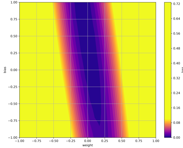
Figure 3: Countour Map of L(w, b)
