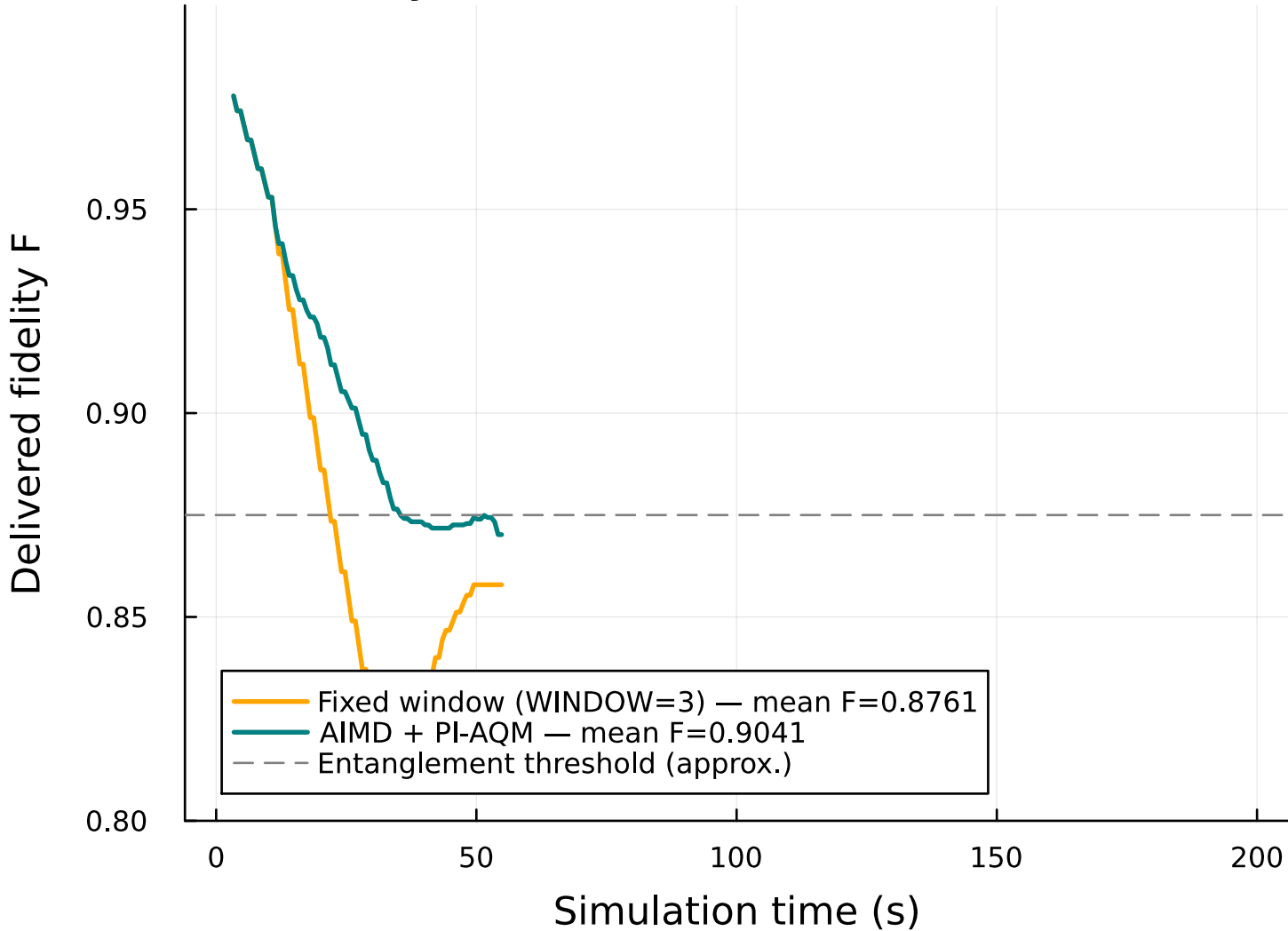
(a) Fidelity over time — 5-node chain, 6 flows
