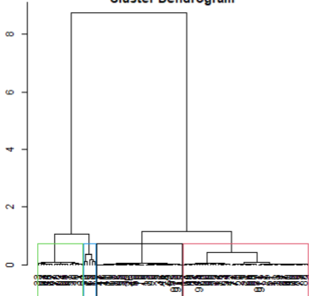
Cluster Dendrogram
