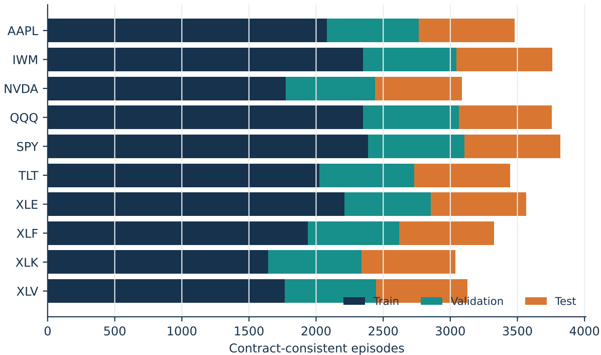
Historical panel after chronological splitting and embargo
