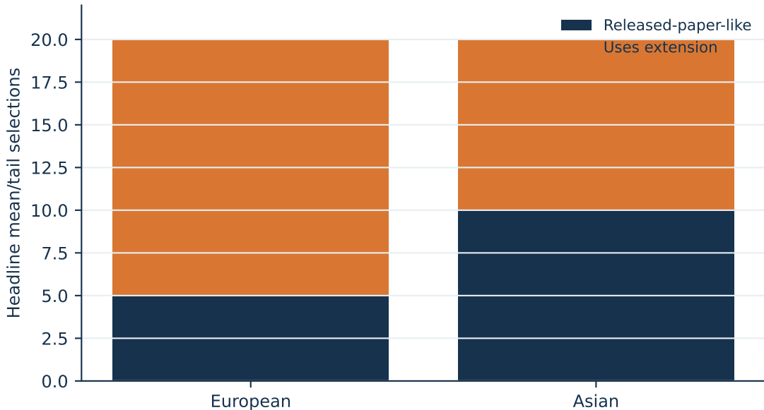
Scope of the validation-selected historical ProtoHedge family
