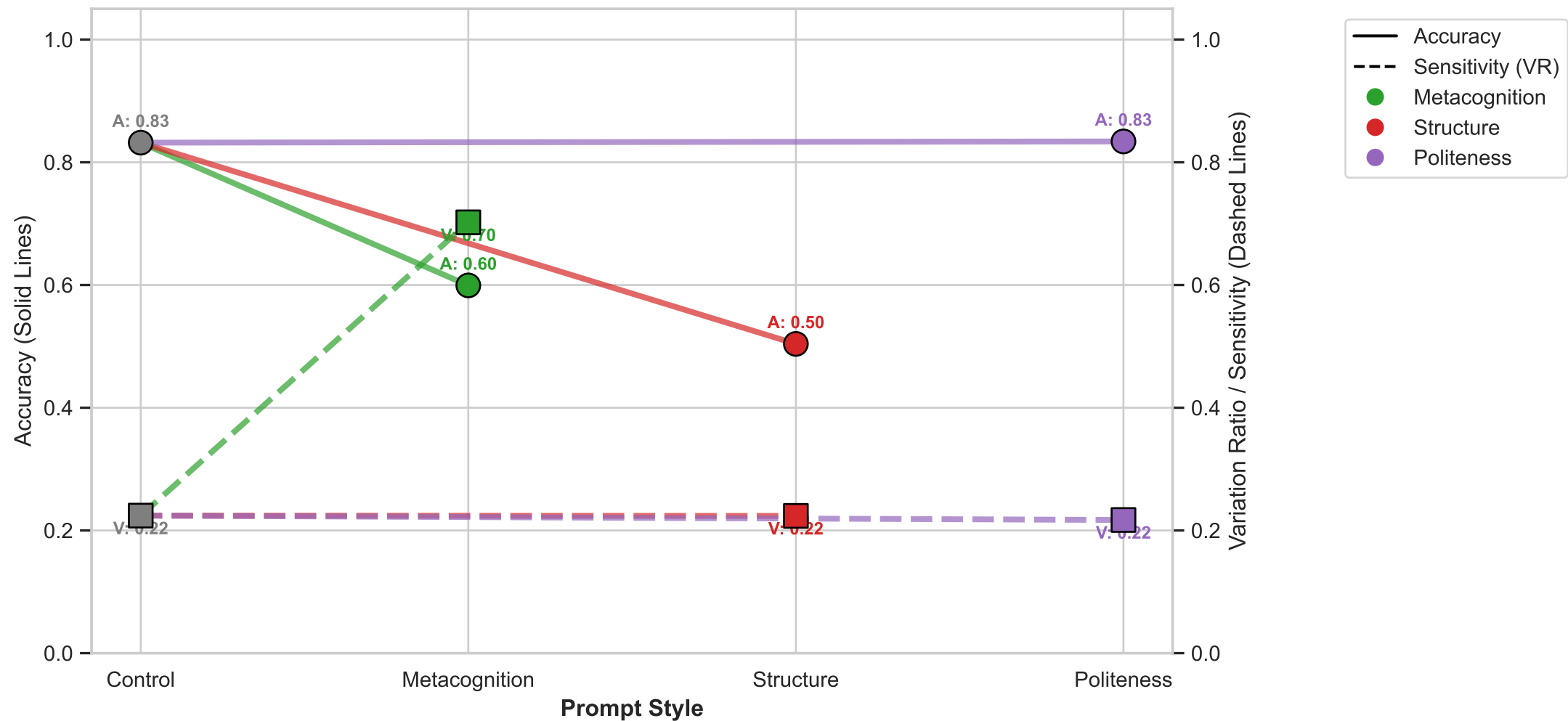
PHASE_6: FLAN-T5-LARGE on CSQA (Totals) Impact of Prompt Attributes relative to Control
