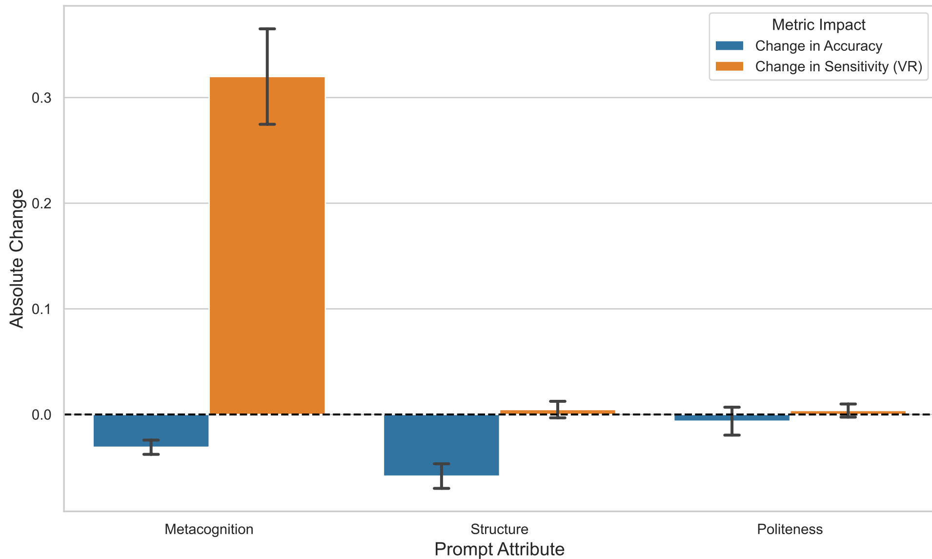
Global Summary (PHASE_6) (Totals - FLAN-T5-BASE): Average Impact of Prompt Attributes Relative to Control Baseline (N=72)
