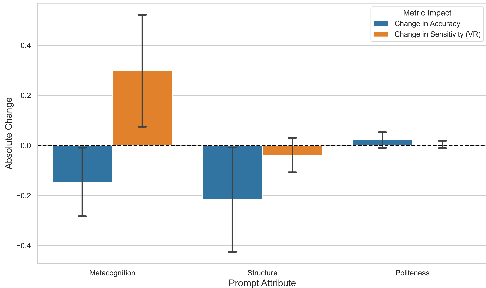
Global Summary (PHASE_6) (Totals - FLAN-T5-LARGE): Average Impact of Prompt Attributes Relative to Control Baseline (N=105)
