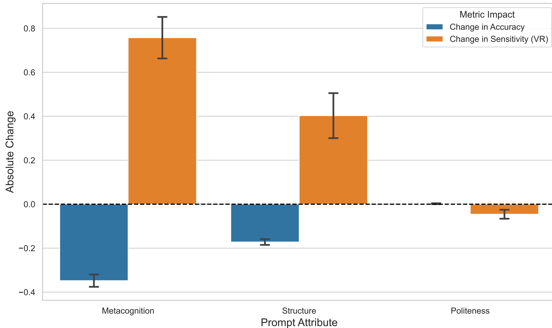
Global Summary (PHASE_6) (Totals - LLAMA-3.2-1B-INSTRUCT): Average Impact of Prompt Attributes Relative to Control Baseline (N=36)
