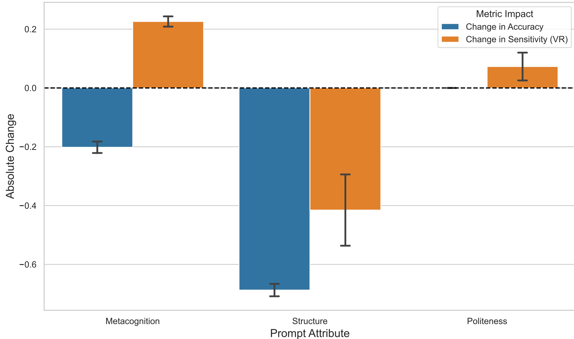
Global Summary (PHASE_6) (Totals - LLAMA-3.2-1B): Average Impact of Prompt Attributes Relative to Control Baseline (N=36)
