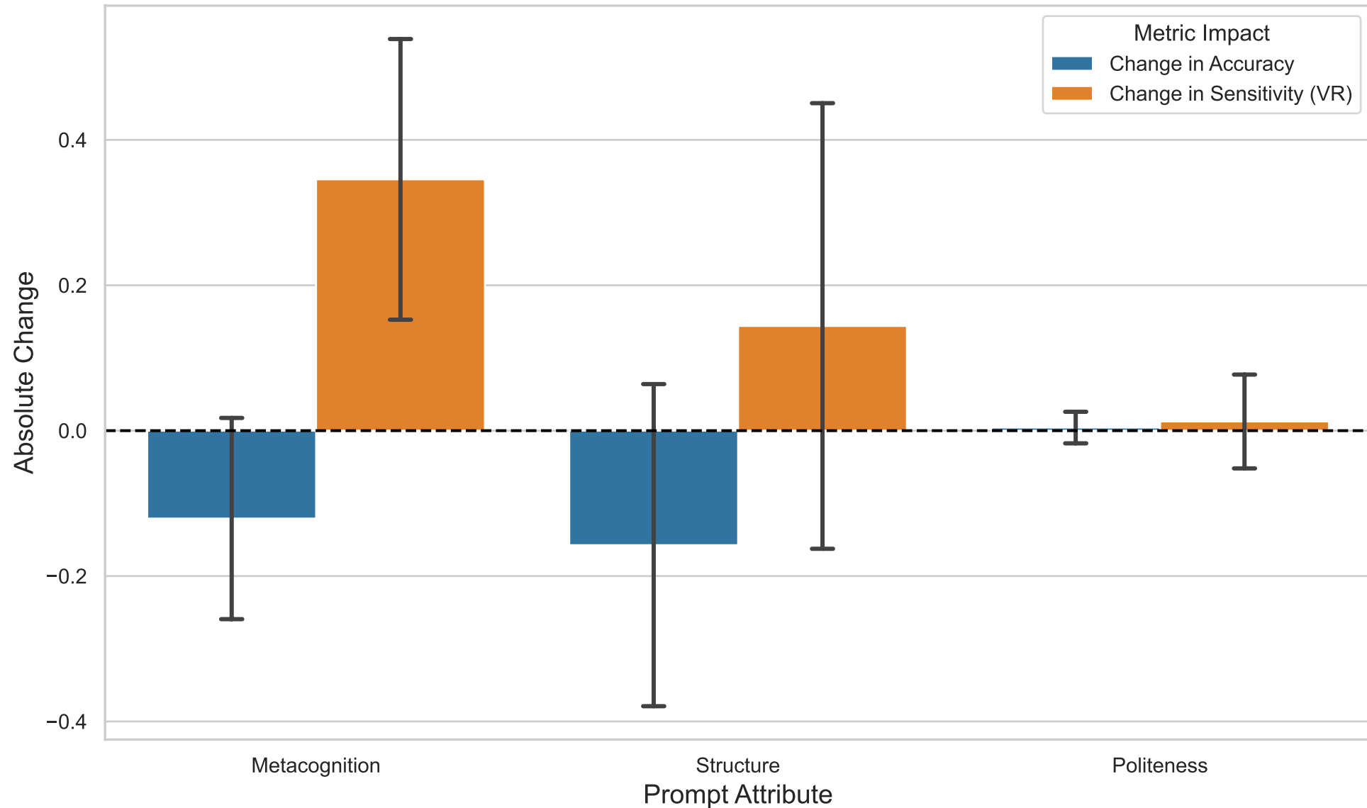
Global Summary (PHASE_6) (Synonyms): Average Impact of Prompt Attributes Relative to Control Baseline (N=285)
