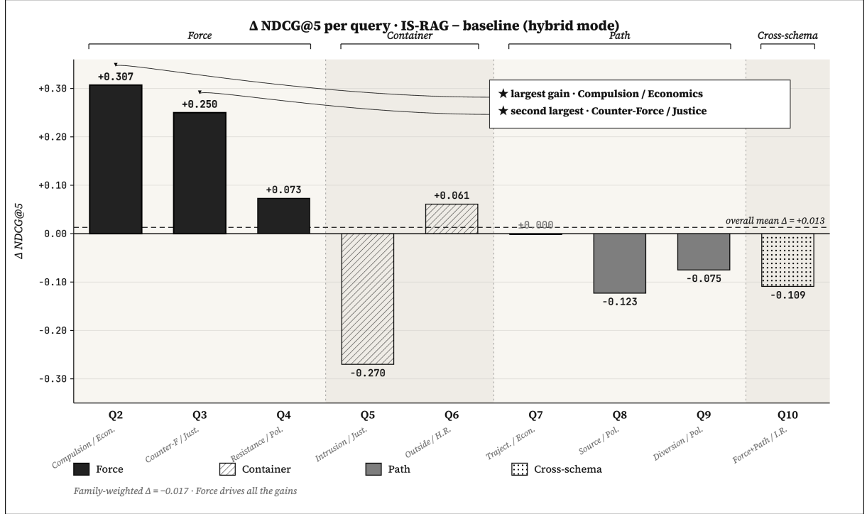
Figure 2: Per-query \Delta NDCG@5 (IS-RAG – baseline).
