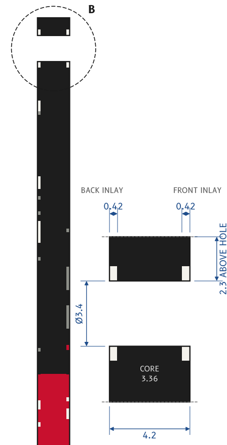
SECTION A-A SCALE 2:1 DETAIL B HOLE AND LAYER STACK, SCALE 5:1
