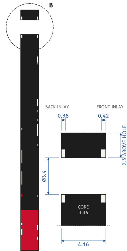
DETAIL B HOLE AND LAYER STACK, SCALE 5:1 SECTION A-A SCALE 2:1
