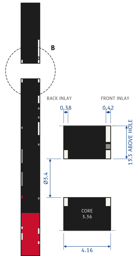
DETAIL B HOLE AND LAYER STACK, SCALE 5:1 SECTION A-A SCALE 2:1
