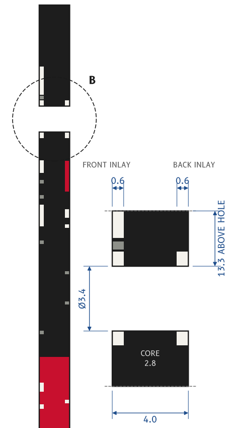
DETAIL B HOLE AND LAYER STACK, SCALE 5:1 SECTION A-A SCALE 2:1
