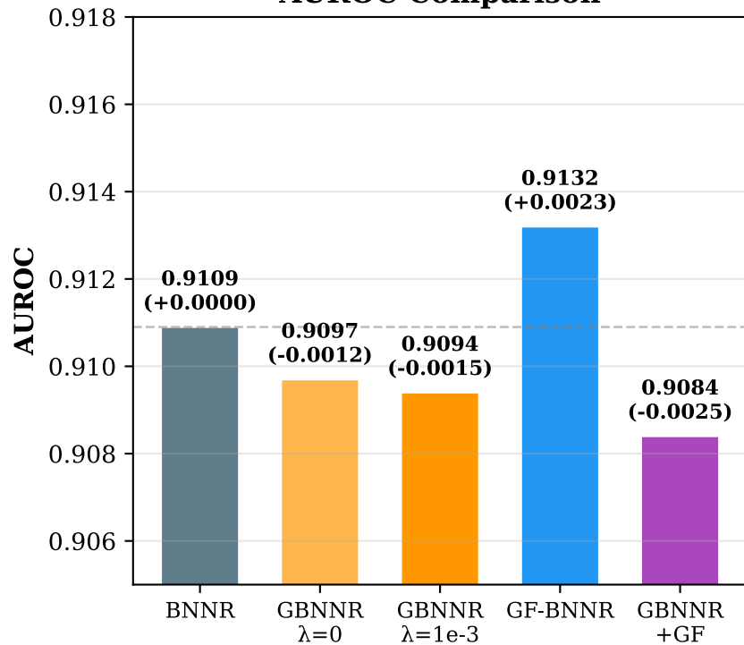
AUROC Comparison
