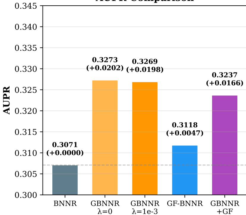
AUPR Comparison
