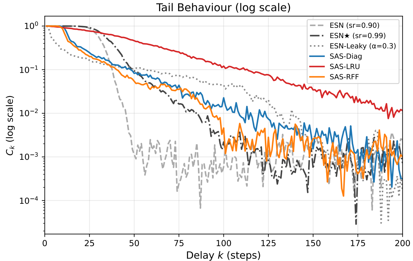
Memory Capacity (N=100, 5 seeds)
