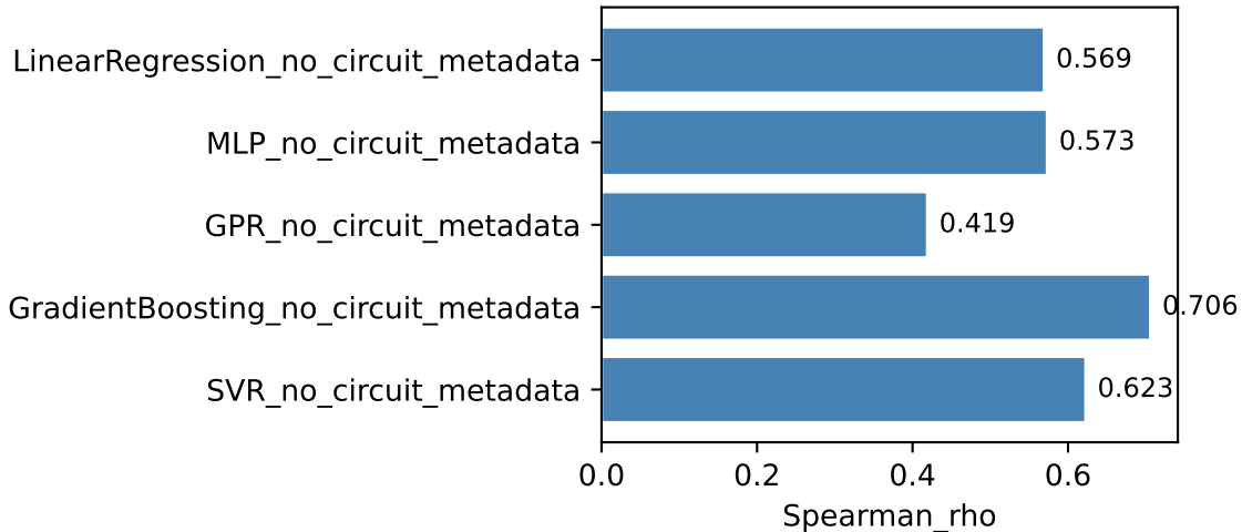
Model comparison — Spearman_rho
