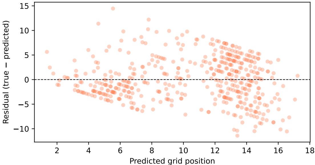
GradientBoosting_no_weather_no_fp: Residual Plot
