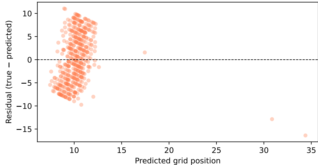
LinearRegression_fp_only: Residual Plot
