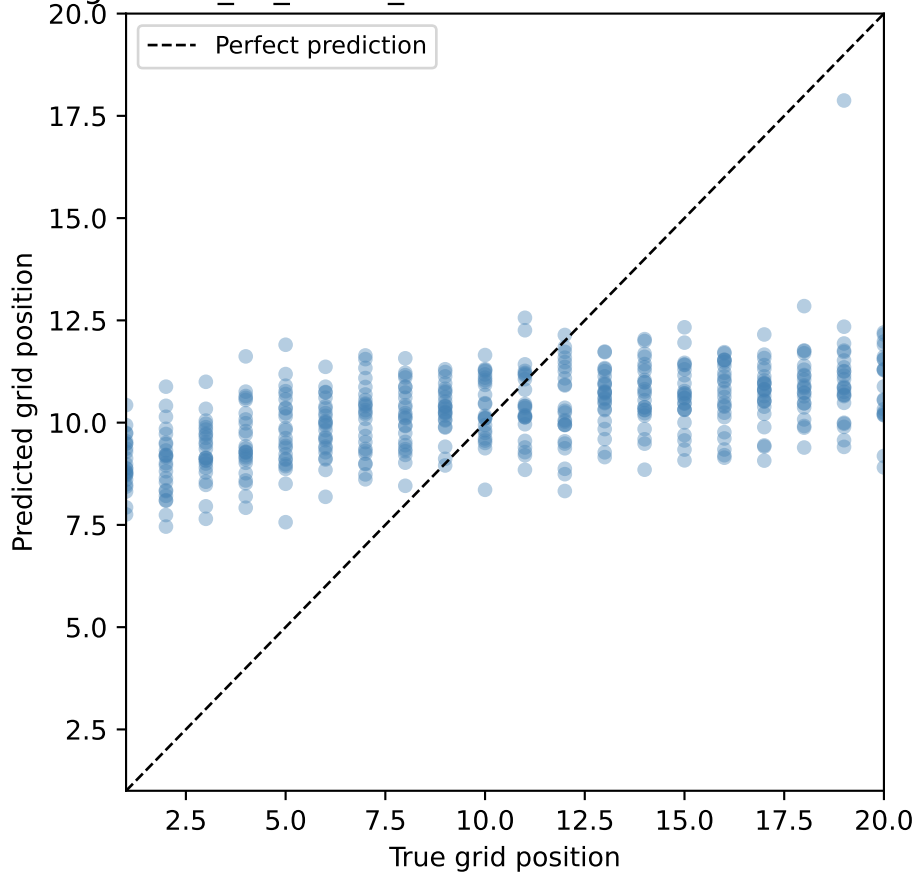
LinearRegression_no_circuit_metadata: Predicted vs True Grid Position
