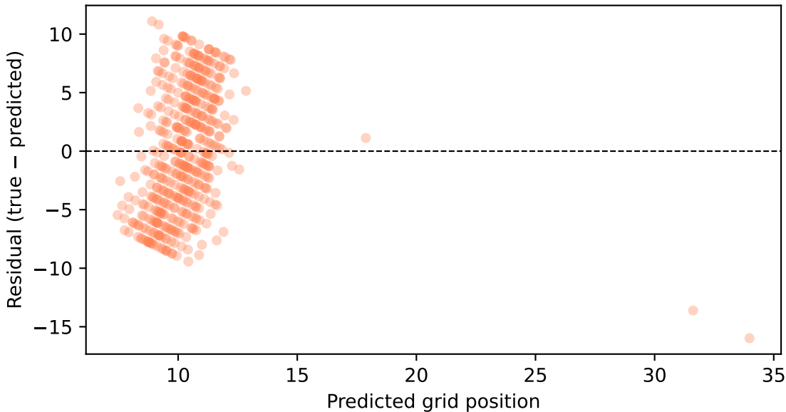
LinearRegression_no_circuit_metadata: Residual Plot
