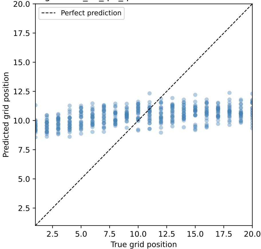
LinearRegression_no_fp1_fp2: Predicted vs True Grid Position
