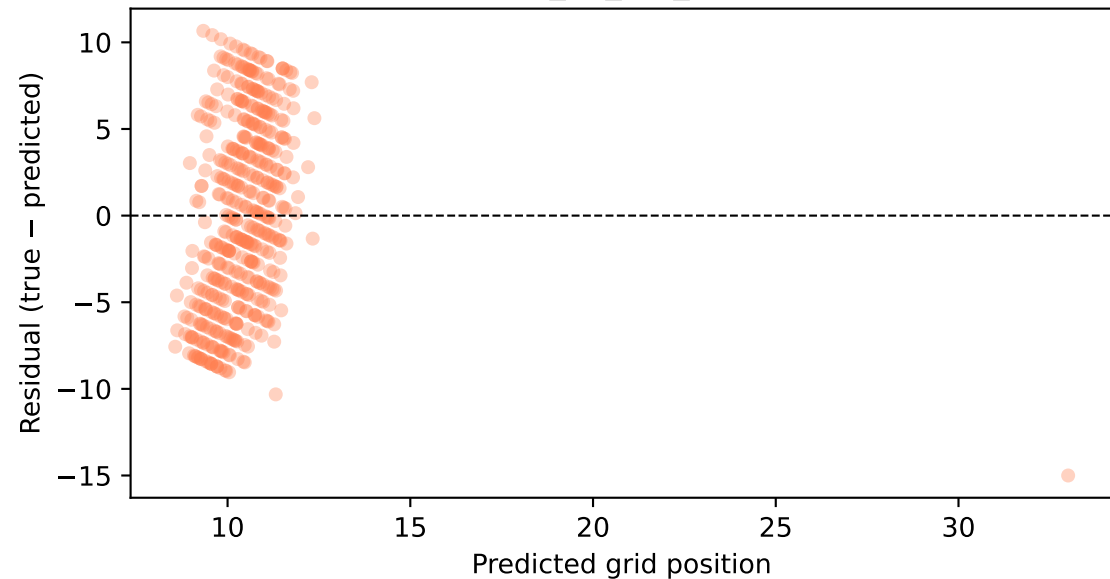
LinearRegression_no_fp1_fp2: Residual Plot
