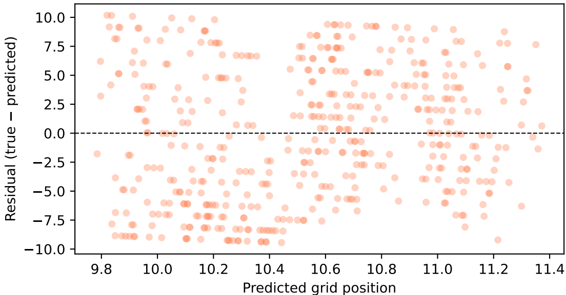
LinearRegression_no_weather_no_fp: Residual Plot
