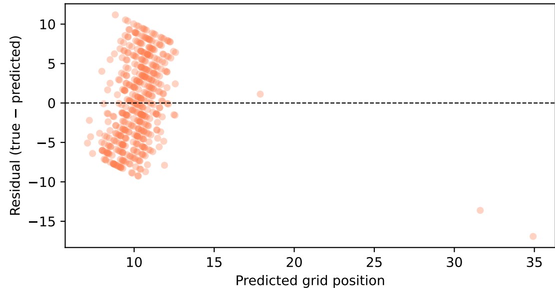
LinearRegression: Residual Plot
