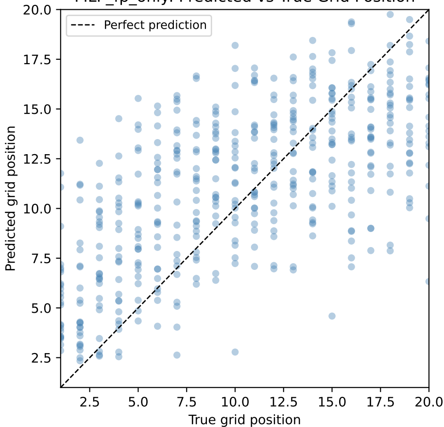
MLP_fp_only: Predicted vs True Grid Position
