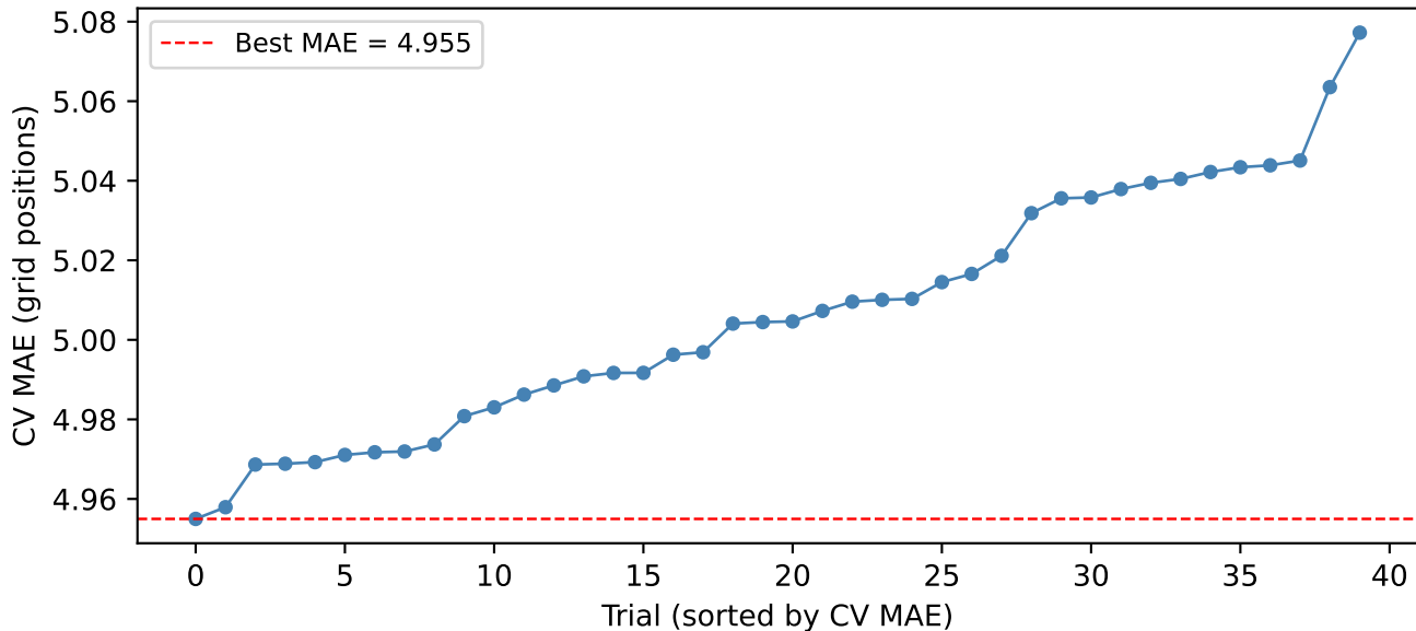
MLP_weather_only: Hyperparameter Search Results
