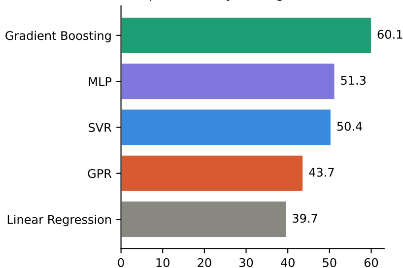
Top-3 accuracy (% , higher is better)
