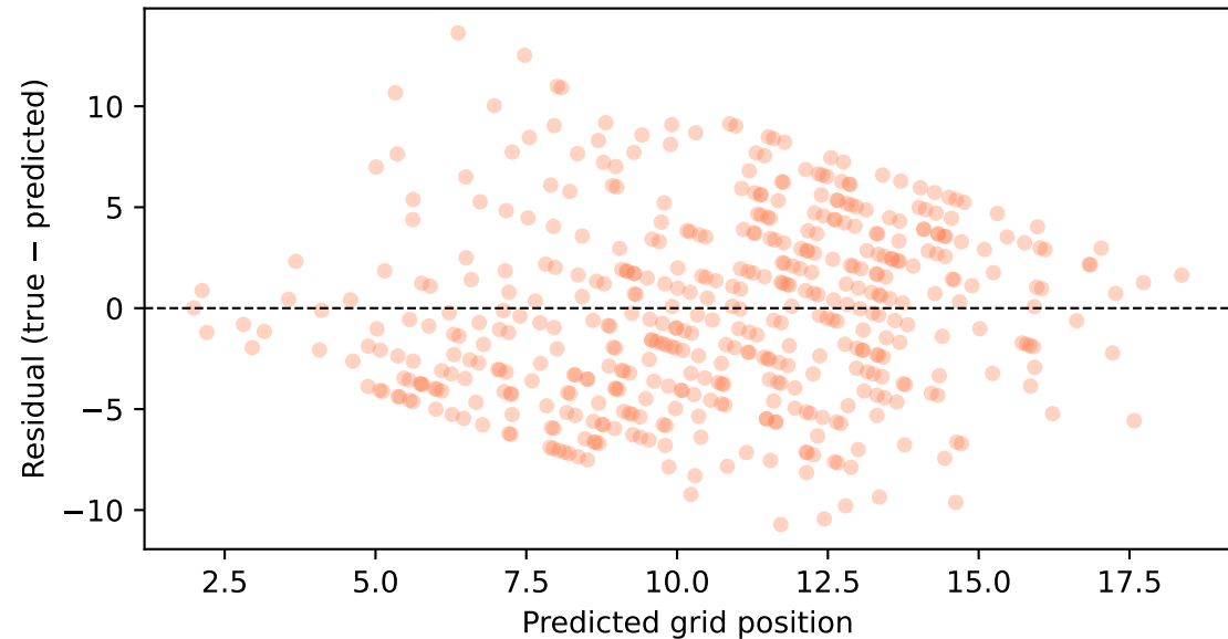
SVR_no_circuit_metadata: Residual Plot
