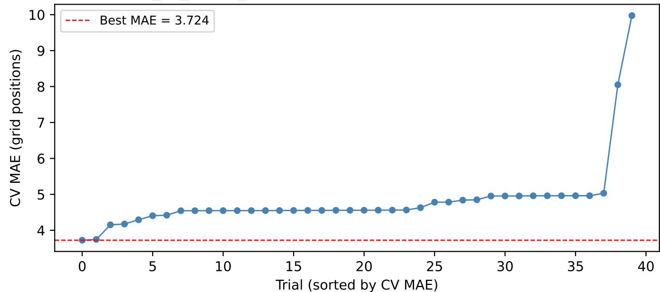
SVR_no_circuit_metadata: Hyperparameter Search Results
