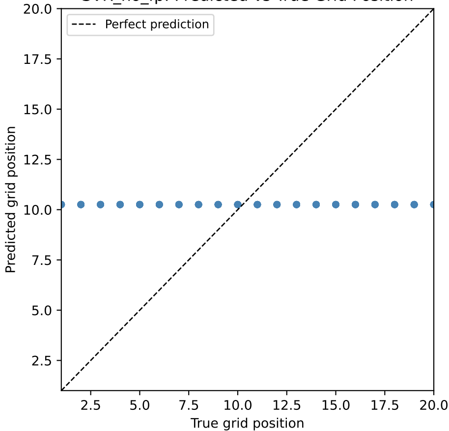
SVR_no_fp: Predicted vs True Grid Position
