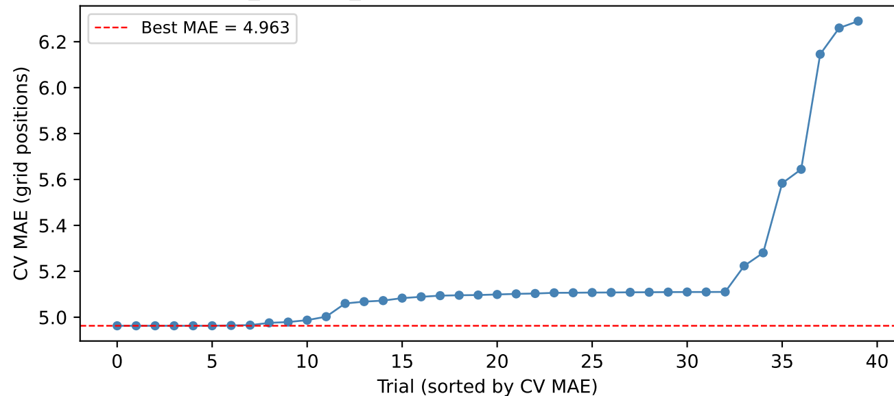
SVR_weather_only: Hyperparameter Search Results
