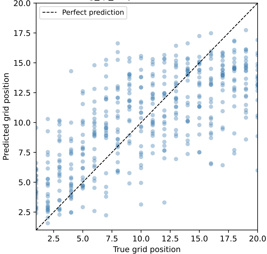
GradientBoosting_fp_only: Predicted vs True Grid Position
